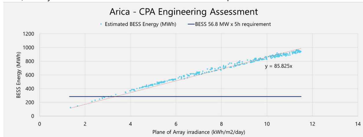
Figure 1: BESS Energy as a function of Plane of Array irradiance
