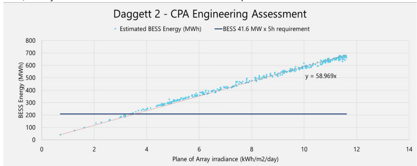
Figure 1: BESS Energy as a function of Plane of Array irradiance
